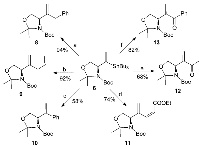
Scheme 3. Cross coupling reactions of stannylated amino alcohol derivative 6 . General reaction conditions: 2 mol-% [(\text{allyl})\text{PdCl}]_2 , 4 mol-% \text{PPh}_3 , 2 equiv. halide, THF, 60 °C, overnight; a) \text{BnBr} ; b) Allyl bromide; c) \text{PhI} ; d) (Z)-ethyl 3-iodoacrylate; e) acetyl chloride; f) \text{PhCOCl} .
