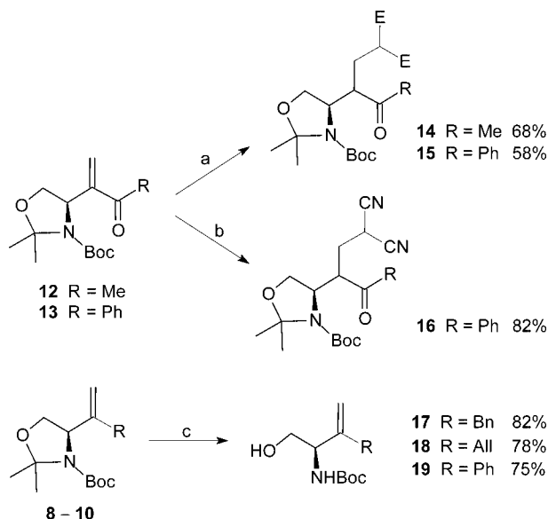
Scheme 4. Modifications of cross coupling products. Reaction conditions: a) \text{CH}_2(\text{COOEt})_2 (2 equiv.), \text{LiI} (2 equiv.), DME, \Delta , 24 h; b) \text{CH}_2(\text{CN})_2 (2 equiv.), \text{LiI} (2 equiv.), DME, \Delta , 24 h; c) 1) 20 mol-% p\text{TsOH} , MeOH, \text{H}_2\text{O} , \Delta , 48 h; 2) \text{NEt}_3 (1 equiv.), \text{Boc}_2\text{O} (1 equiv.).
