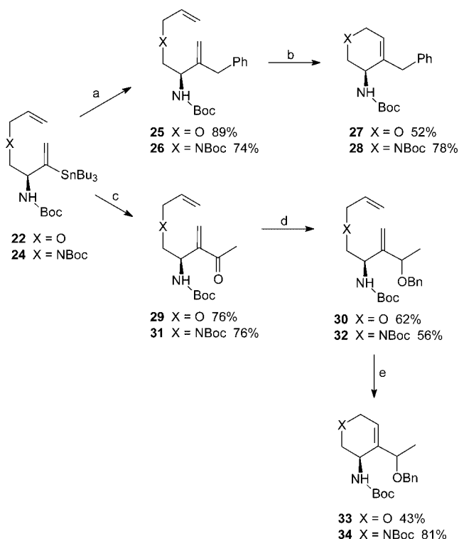
Scheme 6. Synthesis of unsaturated heterocycles via ring closing metathesis. Reaction conditions: (a) BnBr, Pd(PPh 3 ) 4 (2 mol-%), THF, 60 °C, overnight; (b) Grubbs II catalyst, (20 mol-%), CH 2 Cl 2 , room temp., 2 d; (c) acetyl chloride, [(allyl)PdCl] 2 (2 mol-%), PPh 3 (4 mol-%), THF, 60 °C, 16 h; (d) 1) NaBH 4 , CeCl 3 ·7H 2 O, MeOH, 10 min; 2) PhCH 2 Br, Bu 4 NI, NaH, THF, room temp., 16 h.
