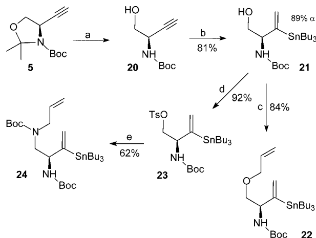
Scheme 5. Synthesis and conversions of stannylated amino alcohol 20 . Reaction conditions: a) 1) 20 mol-% p TsOH, MeOH, H 2 O, \Delta , 48 h; 2) NEt 3 (1 equiv.), Boc 2 O (1 equiv.); b) Bu 3 SnH (3 equiv.), hydroquinone (10 mol-%), Mo(CO) 3 (CN t Bu) 3 (2 mol-%), THF, 55 °C, 16 h; c) 1) NaH, DMF, 0 °C, 30 min; 2) allyl bromide, room temp., 3 h; (d) TsCl, NEt 3 , THF, \Delta , 3 h; d) allylamine, \Delta , 5 h.
