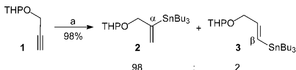
Scheme 1. Hydrostannation of alkyne 1 . Reaction conditions: a) Bu 3 SnH (3 equiv.), hydroquinone (10 mol-%), Mo(CO) 3 (CNtBu) 3 (2 mol-%), THF, 60 °C, 4 h.
