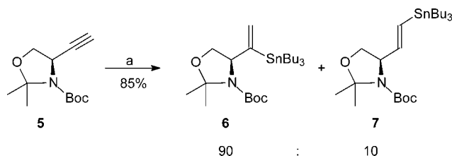
Scheme 2. Hydrostannation of alkyne 5 . Reaction conditions: (a) \text{Bu}_3\text{SnH} (3 equiv.), hydroquinone (10 mol-%), \text{Mo}(\text{CO})_3(\text{CN}t\text{Bu})_3 (2 mol-%), THF, 60 °C, 24 h.
